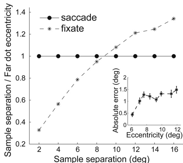
Figure 3. The ratio of separation by eccentricity as a function of that separation. For the 'saccade' (solid line with circles) condition, the eccentricity corresponded directly with the distance between the sample dots. For the 'fixate' (dashed line with asterisks) encoding condition, the eccentricity was calculated as the mean eccentricity of the most peripheral dot of a sample pair of dots. doi:10.1371/journal.pone.0009918.g003
