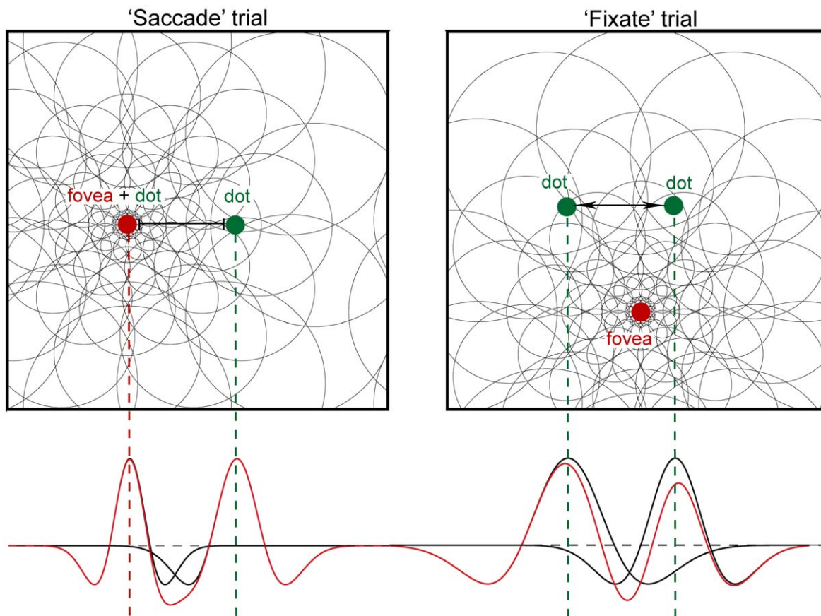
Figure 4. Theoretical neuronal populations response to a pair of dots. The green circles illustrate two sample dots presented on a monitor. The red circles represent gaze position relative to the sample dots. The left panel represents a 'saccade' trial when an observer foveates the leftward dot and at the same time encodes the rightward dot by peripheral vision. The right panel represents a 'fixation' trial when an observer foveates a central cross while both sample dots are encoded by peripheral vision. The empty circles of variable size correspond to receptive fields (RFs) covering visual field. The lower panels characterize neuronal populations responses to the visual stimuli in the 'saccade' (left) and the 'fixate' (right) conditions. The peaks of responses correspond to the positions of the dots when viewed individually (black lines) and when viewed simultaneously (red lines, representing the sum of the functions in black). The line between the sample dots in the 'saccade' condition symbolizes no direct interactions between the neuronal populations (small overlap of RFs). The arrow between the sample dots in the 'fixation' condition signifies a repulsive effect in perceived distance (large overlap of RFs). doi:10.1371/journal.pone.0009918.g004
