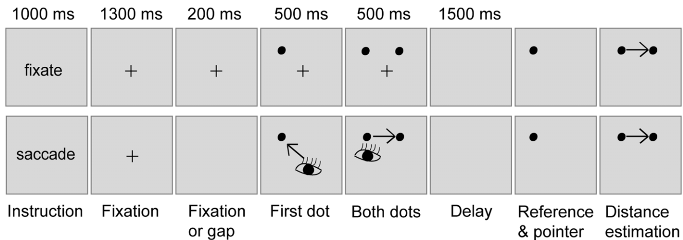
Figure 1. Consecutive stages of 'fixate' and 'saccade' trials. Horizontal separation between two sample dots had to be reproduced after a blank delay period. Distance estimation is based on a stationary reference dot and a movable mouse pointer that appeared on top of each other. The arrows with a depiction of an eye in the 'saccade' trial (lower panel) represent eye movements that brought the sample dots onto the fovea. The arrow in the distance estimation phase indicates a shift of the mouse pointer required to reproduce separation between the sample dots. doi:10.1371/journal.pone.0009918.g001
