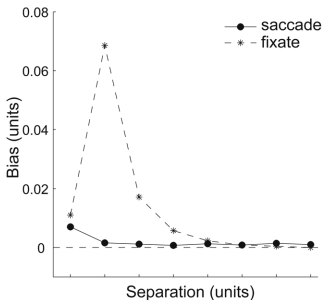
Figure 5. Bias in distance estimation based on the RF sizes predictions. The positive values represent an overestimation of a separation between two dots and the negative values, an underestimation. The difference in the eccentricity-related size of the RFs taxed by the ‘saccade’ (solid line with circles) and ‘fixate’ (dashed line with asterisks) conditions, results in a divergent pattern of distance estimation bias.
