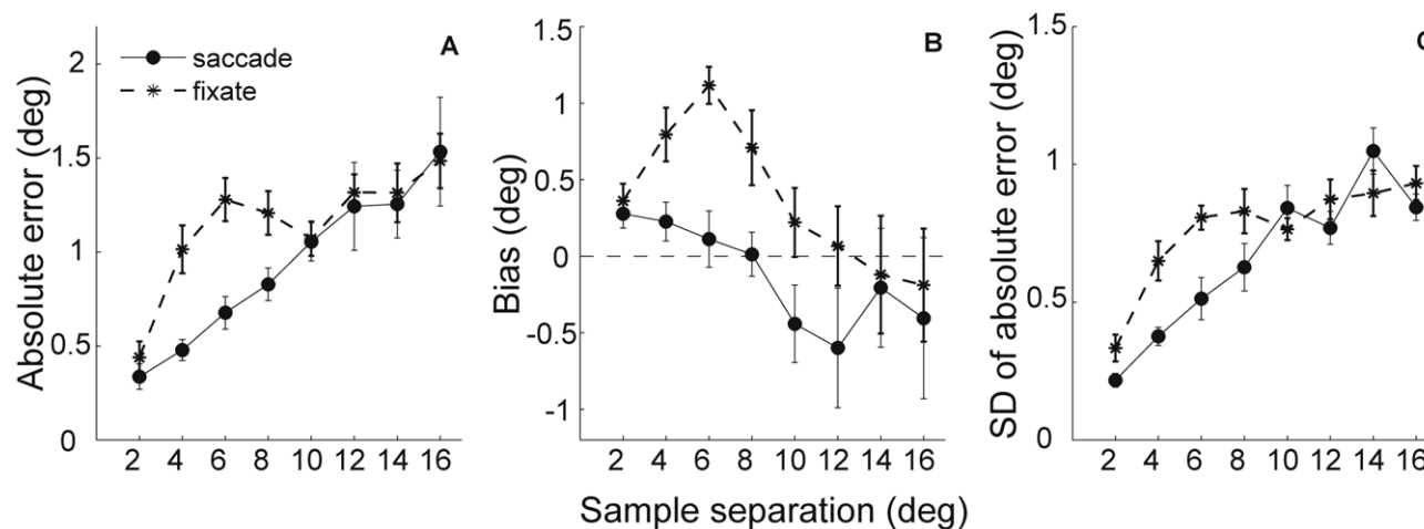
Figure 2. Estimation error as a function of sample distance. A. Absolute estimation error as a function of distance between two sample dots. The two encoding conditions: 'saccade' and 'fixate' (circles with a solid line and asterisks with a dashed line, respectively). B. Estimation bias as a function of sample distance. The sign of the estimation error indicates bias with negative values denoting an underestimation and positive values corresponding to an overestimation of the sample distance. Conventions are the same as in A. C. Standard deviation of the absolute estimation error as a function of separation between the sample dots. Conventions are the same as in A. Error bars denote SEM ( n = 7 ). doi:10.1371/journal.pone.0009918.g002
